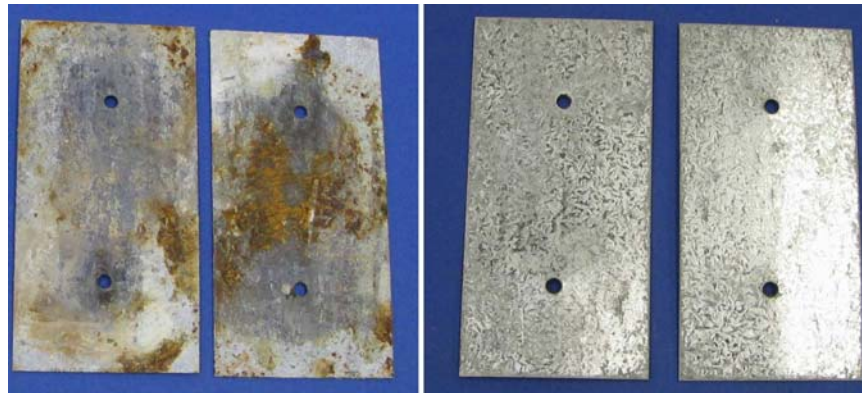
Figure 4. Corrosion of CT G90 with (right) and without (left) the use of barrier protection.
