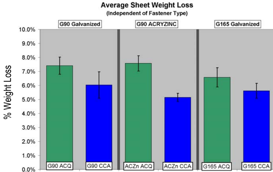
Figure 1. Results of cyclical rainfall/humidity test.
