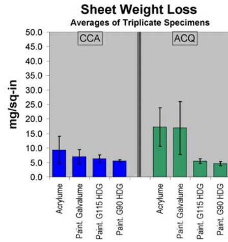
Figure 3. Weight loss of pre-painted sheets.
